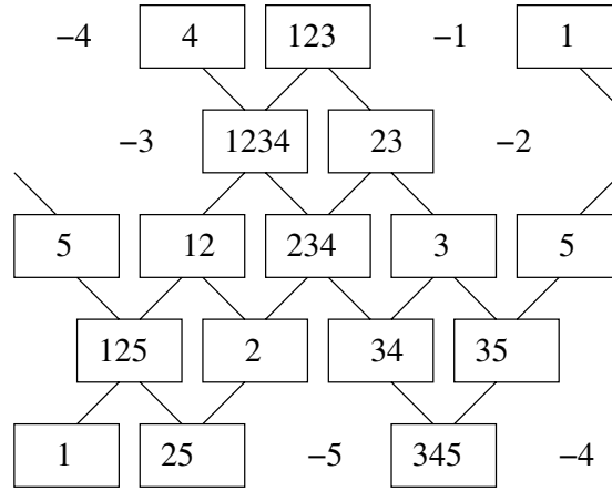
FIGURE 6. Example of Auslander-Reiten quiver
