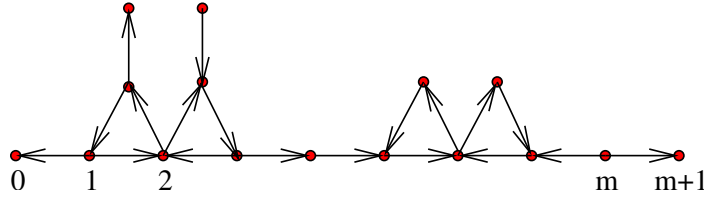
FIGURE 5. Quiver Q and subquiver Q' of type A
